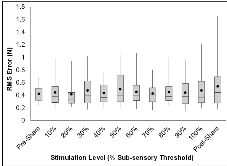
Figure 3. Box plots presenting 1 st quartile, median, and 3 rd quartile force stabilization RMS errors for each stimulation level. Top and bottom whiskers present the max and min RMS errors, respectively, for each stimulation level. The dots indicate the mean RMS error for each stimulation level.
